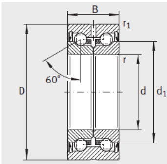
ZKLN...-2RS ZKLN...-2Z
