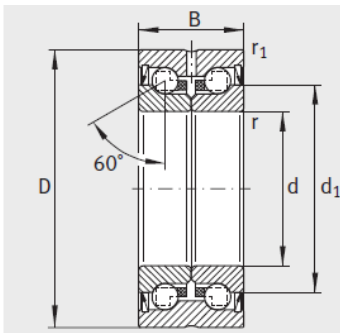
ZKLN...-2RS ZKLN...-2Z
